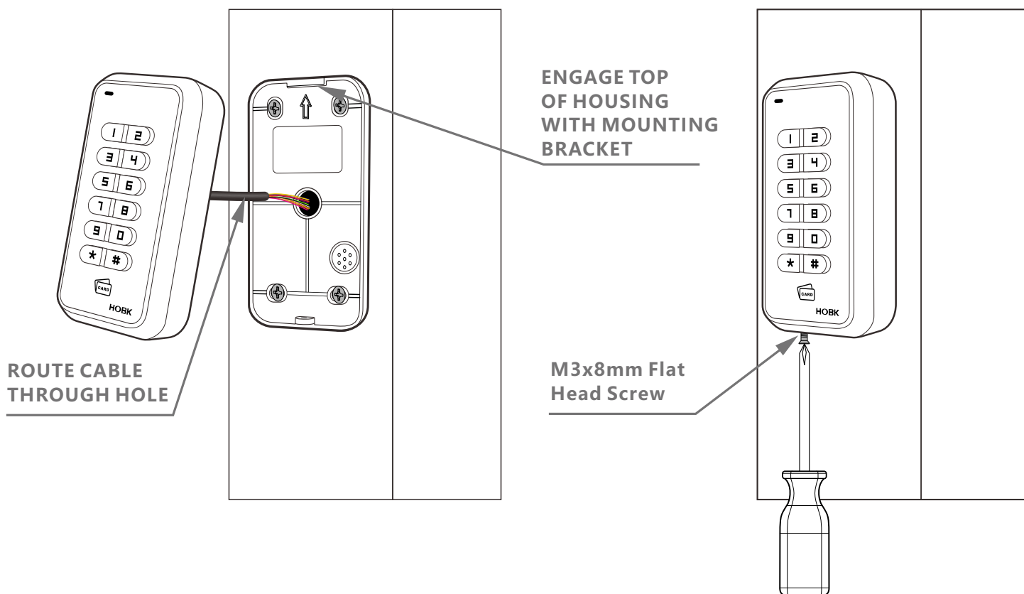
Figure 4 - Installation of HBK-D04K
